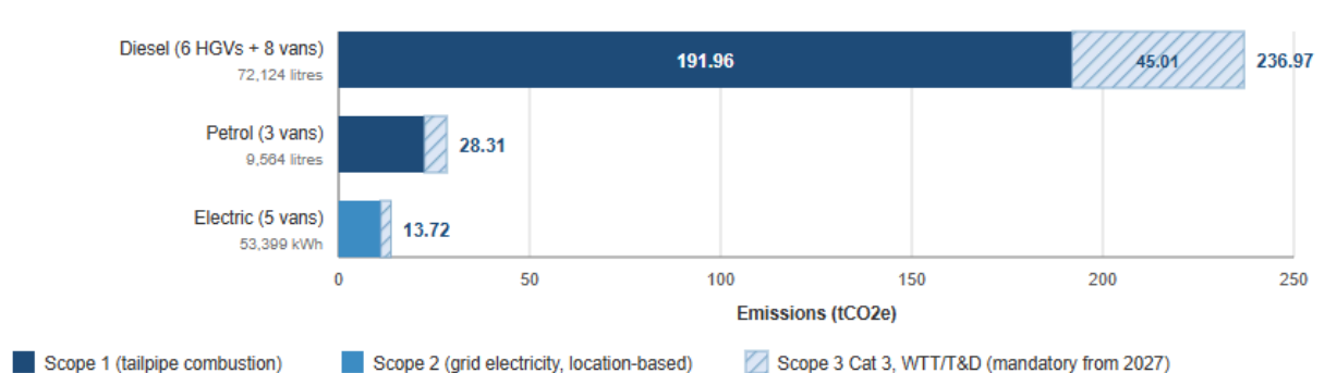
Figure 6.2: Vehicle fleet CO 2 e emissions by fuel type, 2024
